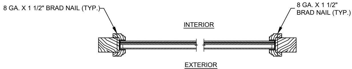
10 4 HORIZONTAL CROSS SECTION SASH SET SIDELITE PANELS
