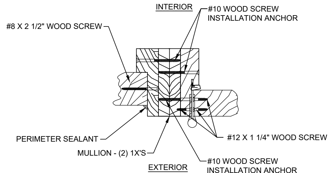
V HORIZONTAL SECTION GLAZED SASH SET SIDELITE PANEL / GLAZED / OPAQUE HINGE STILE DOOR PANEL AT MULLION OUTSWING SHOWN / INSWING OPPOSITE (SEE SHEET 4 SECTIONS 7, 8 & 9 FOR APPROPRIATE DOOR PANELS & SHEET 4 SECTION 10 FOR APPROPRIATE SIDELITE PANEL)
