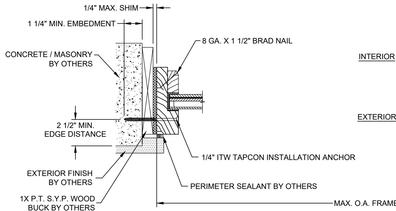
M HORIZONTAL SECTION GLAZED DIRECT SET SIDELITE PANEL AT JAMB CONCRETE / MASONRY SUBSTRATE OUTSWING SHOWN / INSWING OPPOSITE (SEE SHEET 4 SECTION 11 FOR APPROPRIATE SIDELITE SECTION)
