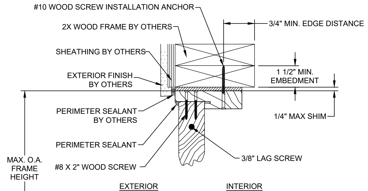
G VERTICAL SECTION GLAZED SIDELITE PANEL AT HEAD WOOD FRAME SUBSTRATE OUTSWING SHOWN / INSWING OPPOSITE (SEE SHEET 3 SECTIONS 2, 4 & 5 FOR APPROPRIATE SIDELITE SECTIONS)
