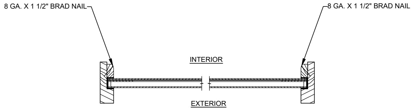
11 4 HORIZONTAL CROSS SECTION DIRECT SET SIDELITE PANELS
