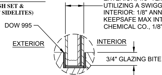
GLAZING DETAIL 2 (FOR SASH SET & DIRECT SET SIDELITES)
