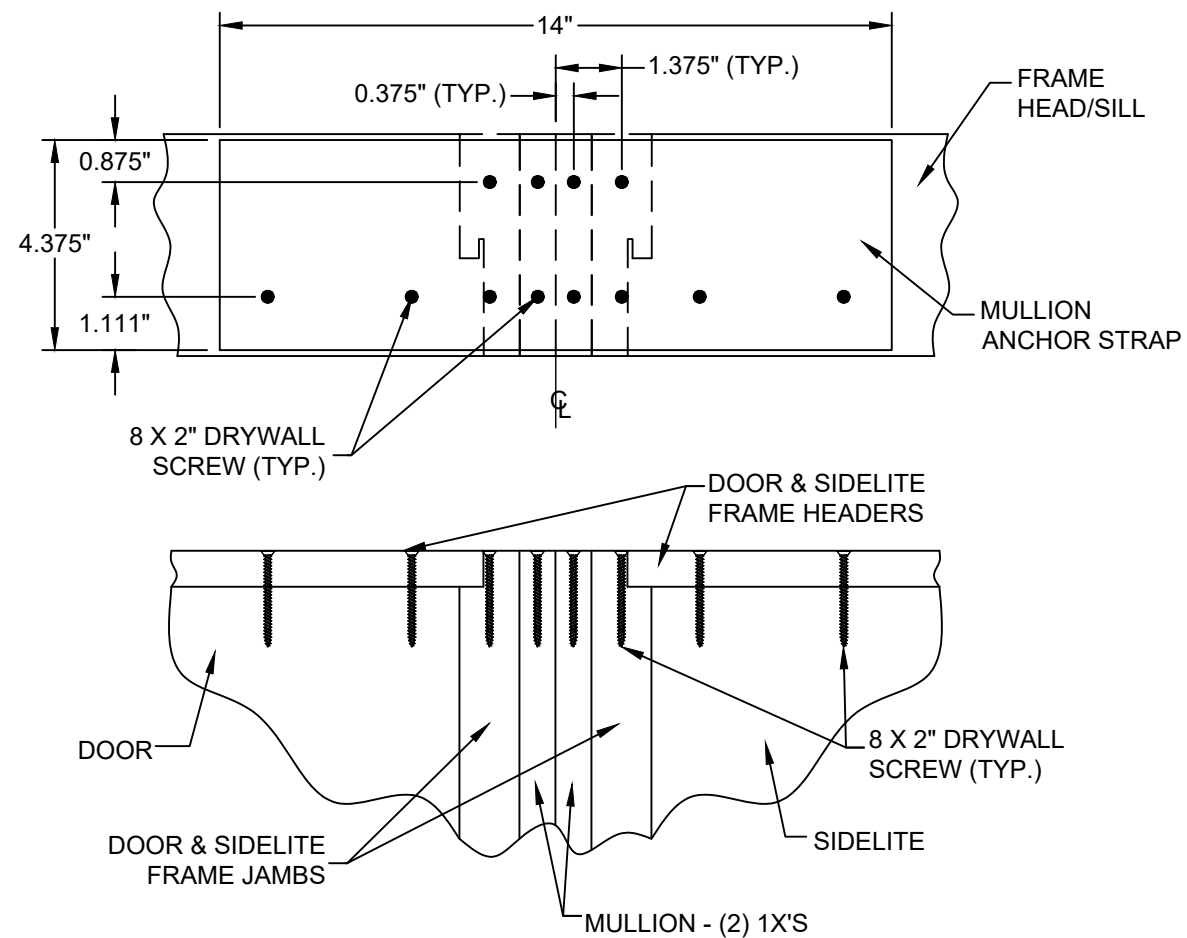
MULLION STRAP ANCHOR DETAIL MULLION @ HEAD & SILL
