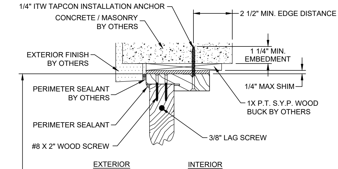
F VERTICAL SECTION GLAZED SIDELITE PANEL AT HEAD CONCRETE / MASONRY SUBSTRATE OUTSWING SHOWN / INSWING OPPOSITE (SEE SHEET 3 SECTIONS 2, 4 & 5 FOR APPROPRIATE SIDELITE SECTIONS)
