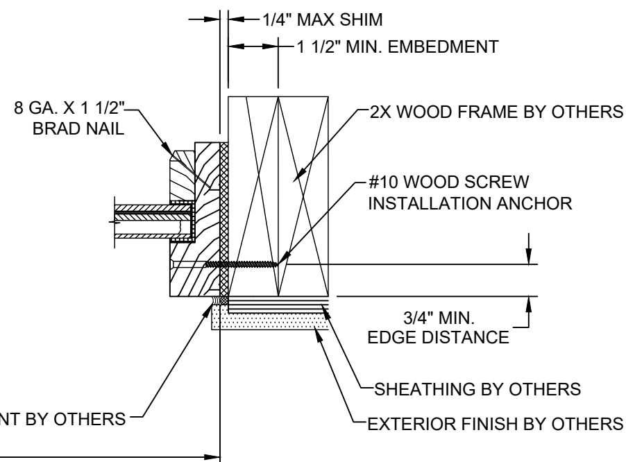
N HORIZONTAL SECTION GLAZED DIRECT SET SIDELITE PANEL AT JAMB WOOD FRAME SUBSTRATE OUTSWING SHOWN / INSWING OPPOSITE (SEE SHEET 4 SECTION 11 FOR APPROPRIATE SIDELITE SECTION)
