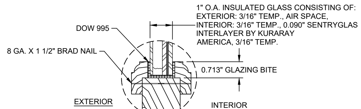
GLAZING DETAIL 2 (FOR SASH SET & DIRECT SET SIDELITES)
