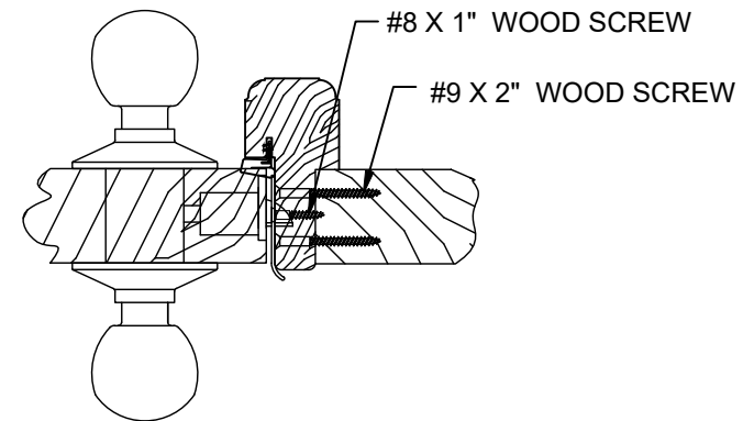
X HORIZONTAL SECTION GLAZED LOCK STILE DOOR PANEL AT ASTRAGAL OUTSWING SHOWN / INSWING OPPOSITE (SEE SHEET 4 SECTIONS 6, 7 & 8 FOR APPROPRIATE DOOR SECTIONS)
